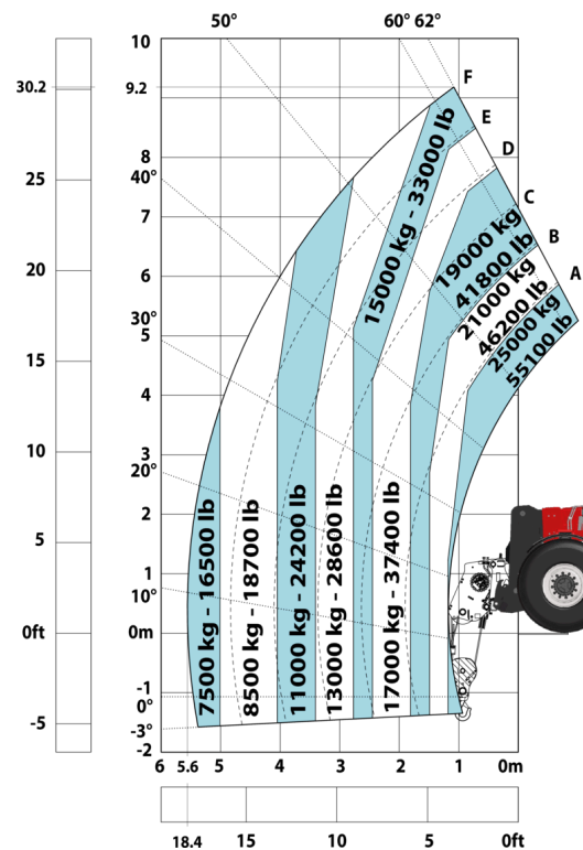
Machine on tires with winch 25000 kg (Metric)
